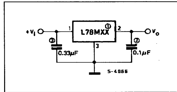
Figure 13 : Fixed Output Regulator.
