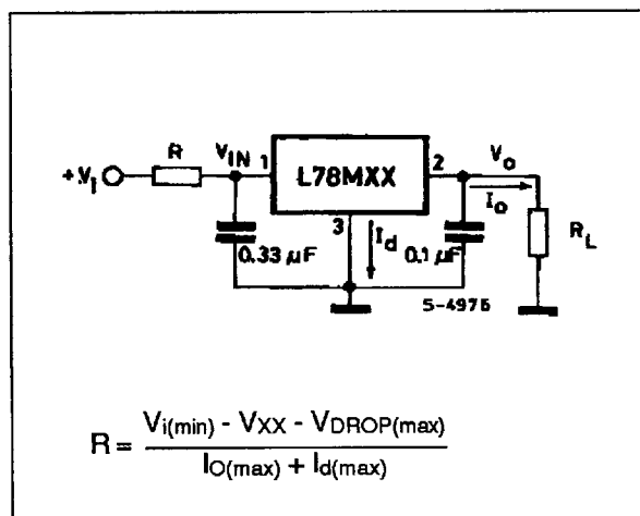
Figure 22 : Reducing Power Dissipation with Dropping Resistor.
