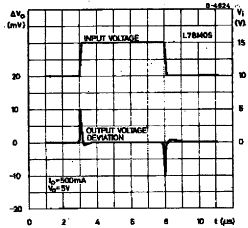
Figure 13 : Fixed Output Regulator.
