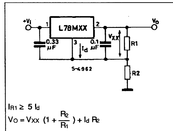
Figure 15 : Circuit for Increasing Output Voltage.
