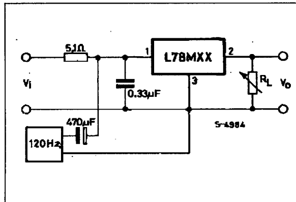
Figure 3 : Ripple Rejection.
