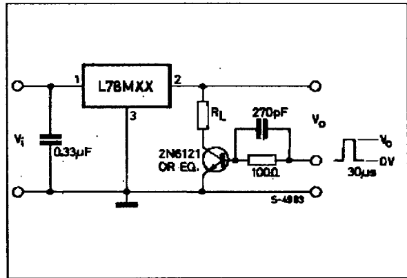
Figure 2 : Load Regulation.
