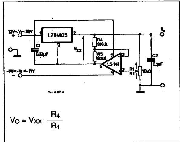
Figure 19 : High Output Current with Short Circuit Protection.
