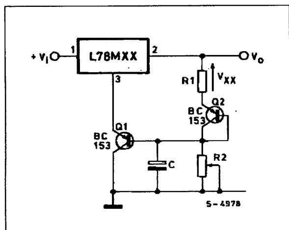
Figure 24 : Adjustable Output Voltage with Temperature Compensation.
