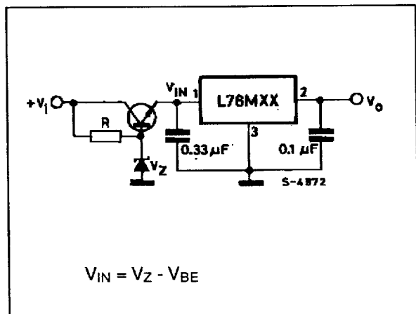
Figure 21 : High Input Voltage Circuit.
