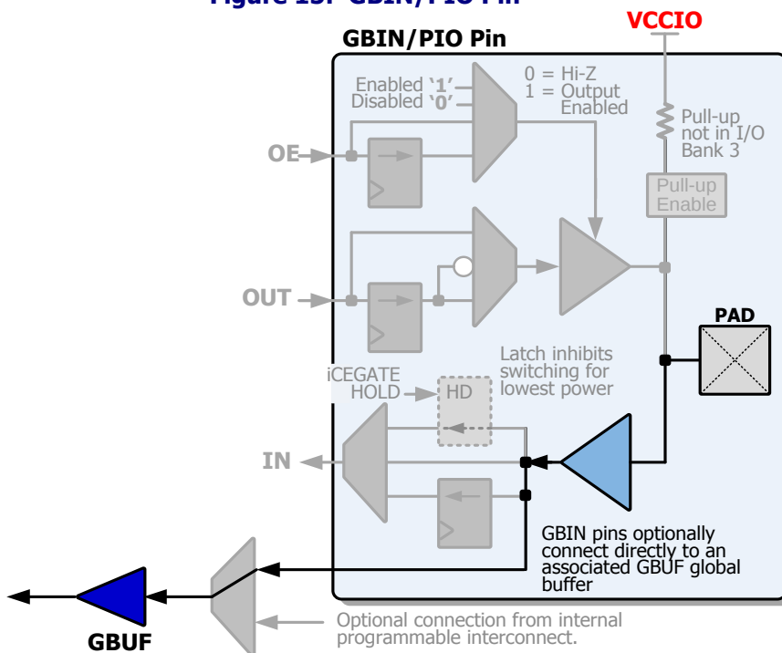
Figure 15: GBIN/PIO Pin
