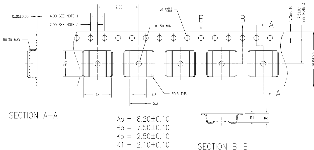
Figure 11. 20-Pin SSOP Carrier Tape Drawing
