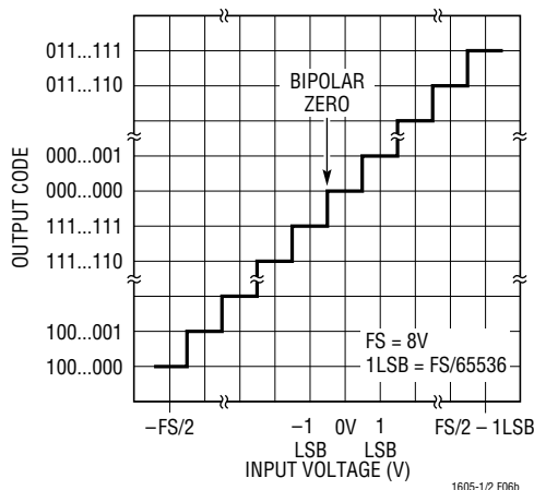
Figure 6B. LTC1605-2 Bipolar Transfer Characteristics
