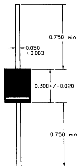
EPOXY CASE
