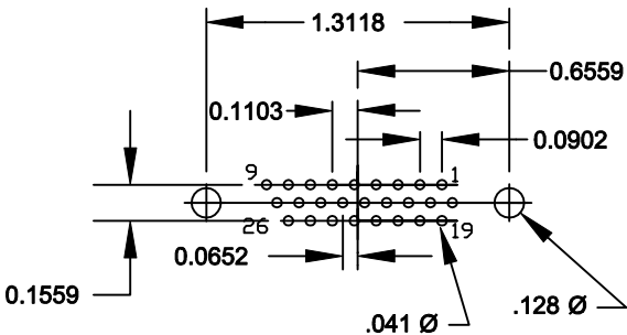
26 POSITION FEMALE
