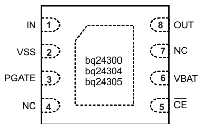
PINOUT
