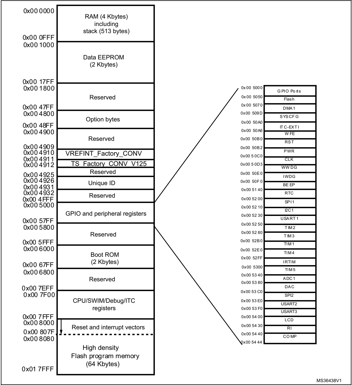
Figure 9. Memory map
