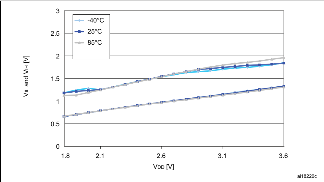
Figure 25. Typical V_{IL} and V_{IH} vs. V_{DD} (standard I/Os)
