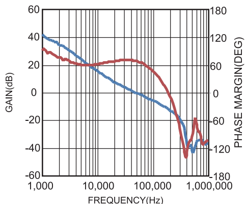
Bode Plot
