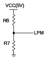
FIGURE 7. LPM Network
