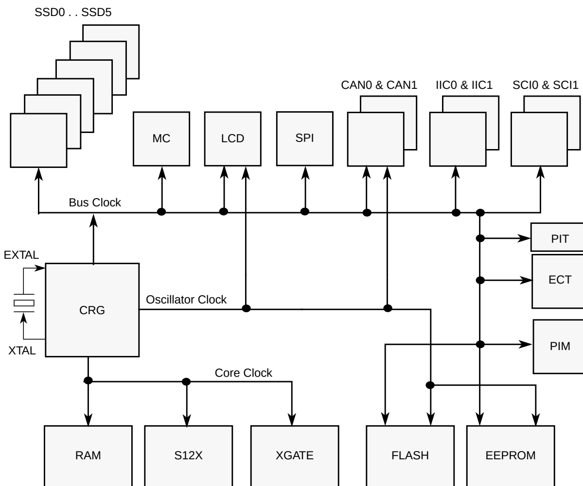
Figure 1-10. Clock Connections
