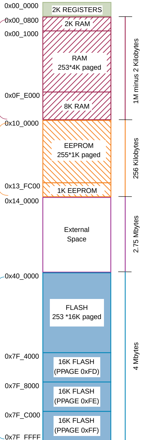
Figure 25-21. Expansion of the Local Address Map
