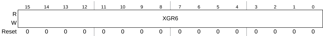
Figure 5-17. XGATE Register 6 (XGR6)
