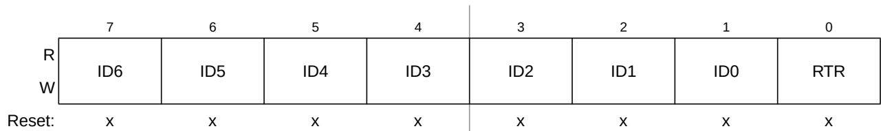
Figure 14-29. Identifier Register 3 (IDR3) — Extended Identifier Mapping
