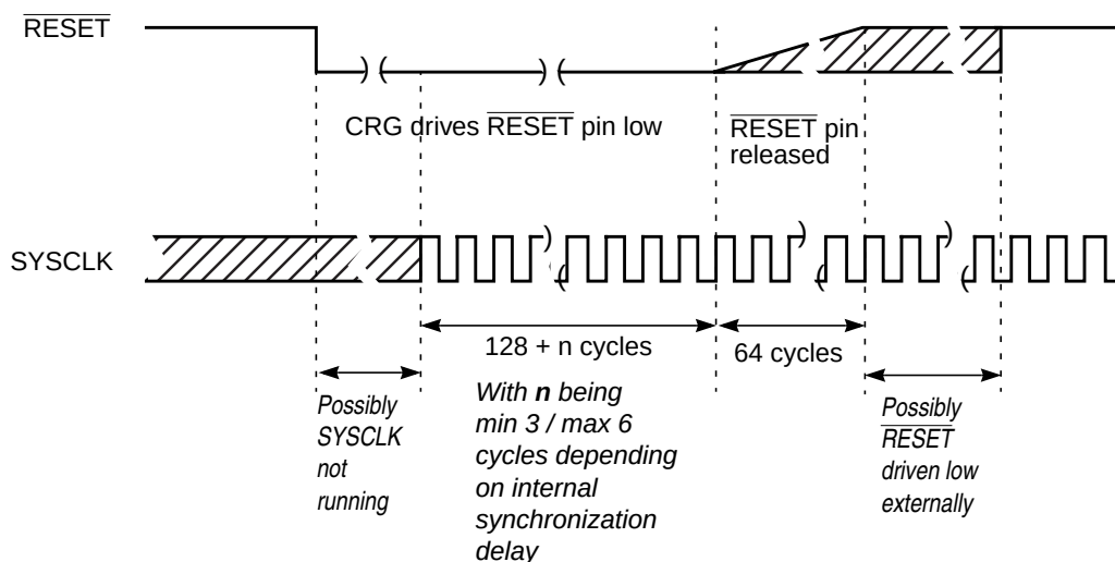
Figure 7-25. RESET Timing
