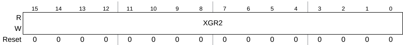
Figure 5-13. XGATE Register 2 (XGR2)
