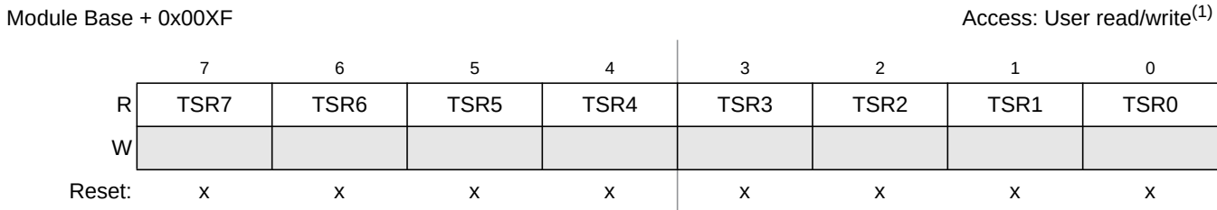
Figure 14-38. Time Stamp Register — Low Byte (TSRL)
