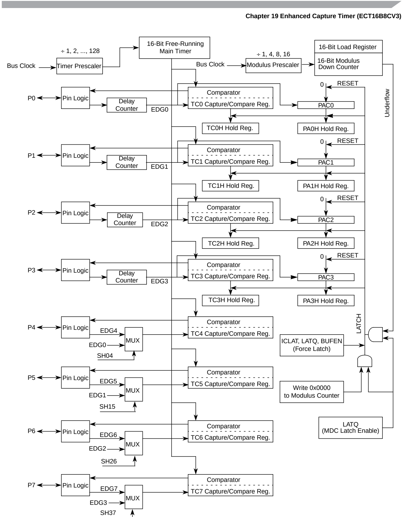
Figure 19-67. Detailed Timer Block Diagram in Latch Mode when PRNT = 0
