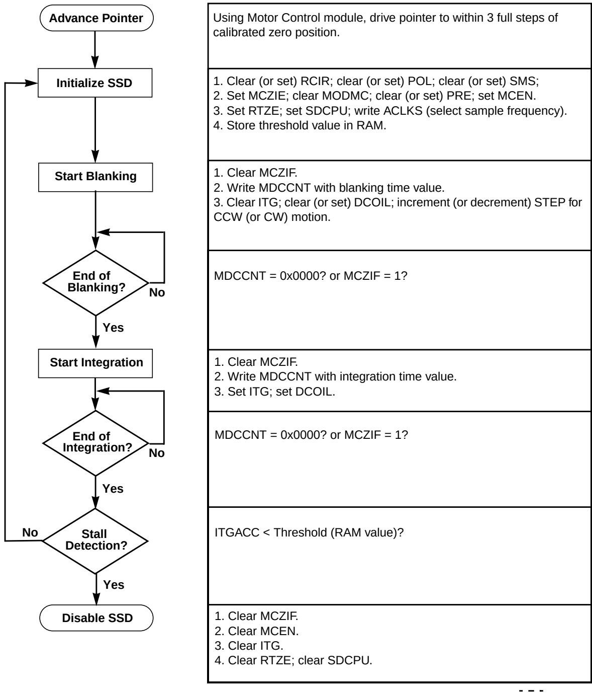
Figure 12-15. Return-to-Zero Flowchart
