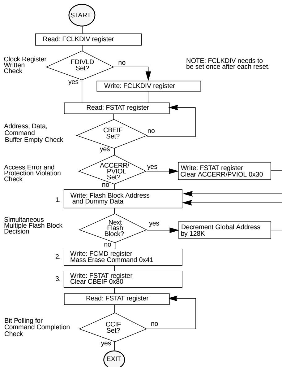
Figure 3-30. Example Mass Erase Command Flow
