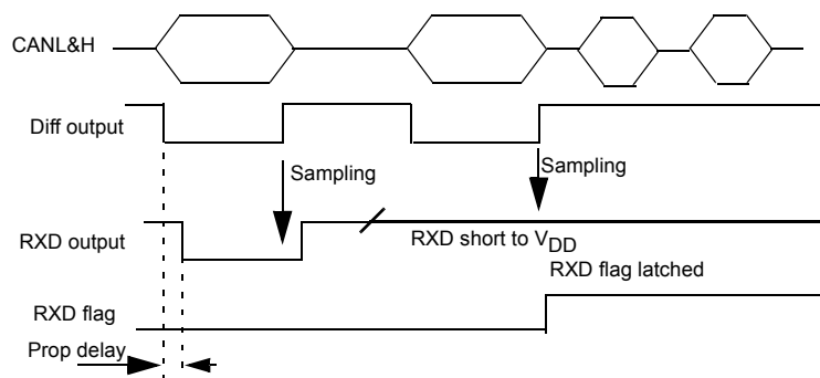
Figure 39. RXD Path Simplified Schematic, RXD Short to V_{DD} Detection
