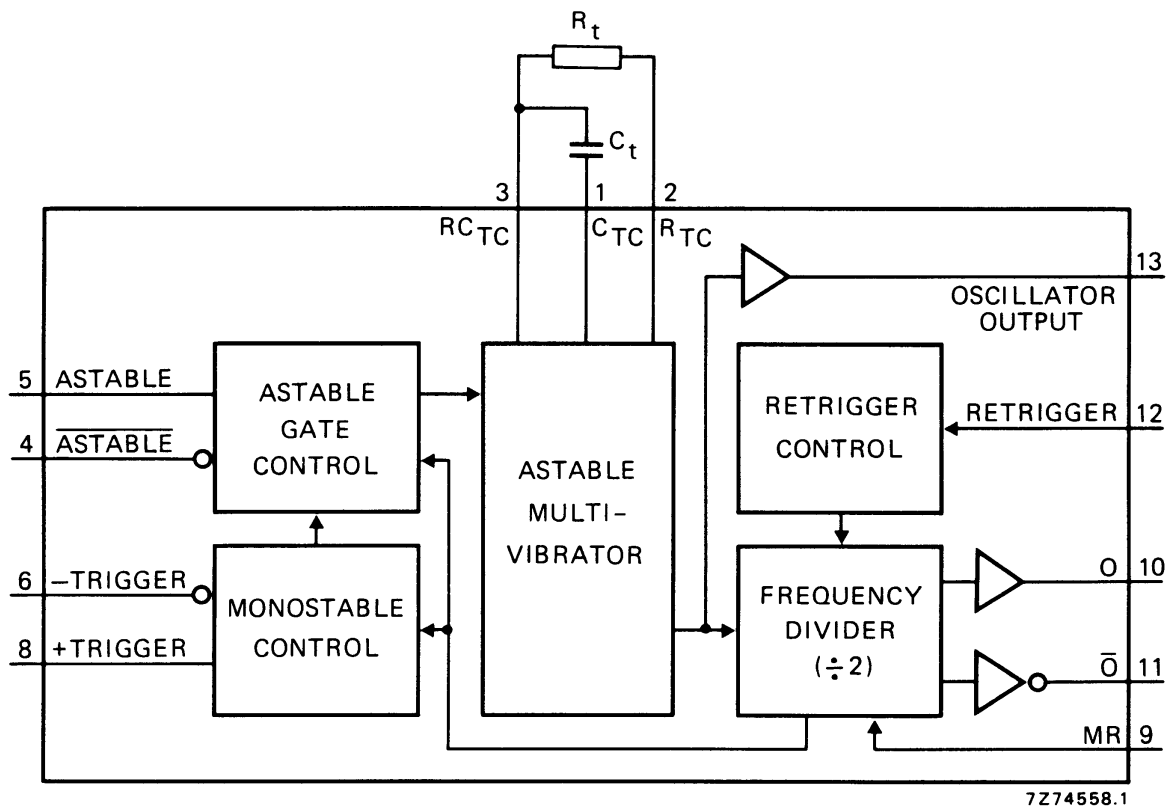
Fig.1 Functional diagram.
