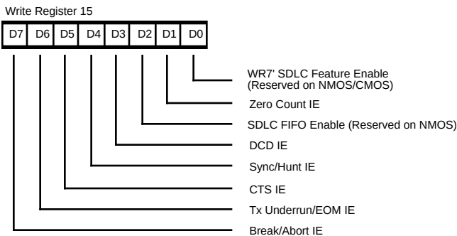
Figure 5-18. Write Register 15
