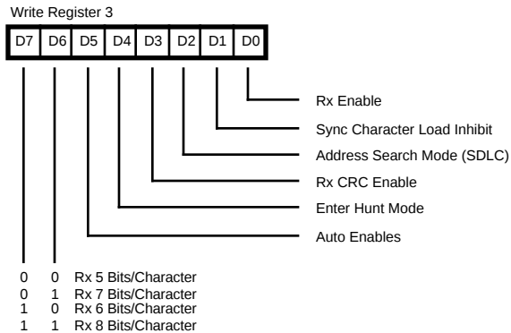
Figure 5-5. Write Register 3
