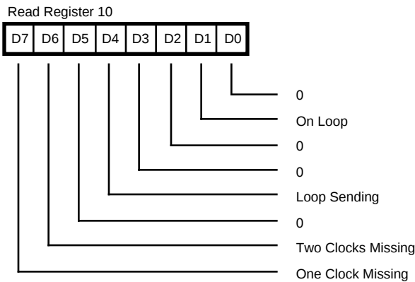
Figure 5-25. Read Register 10
