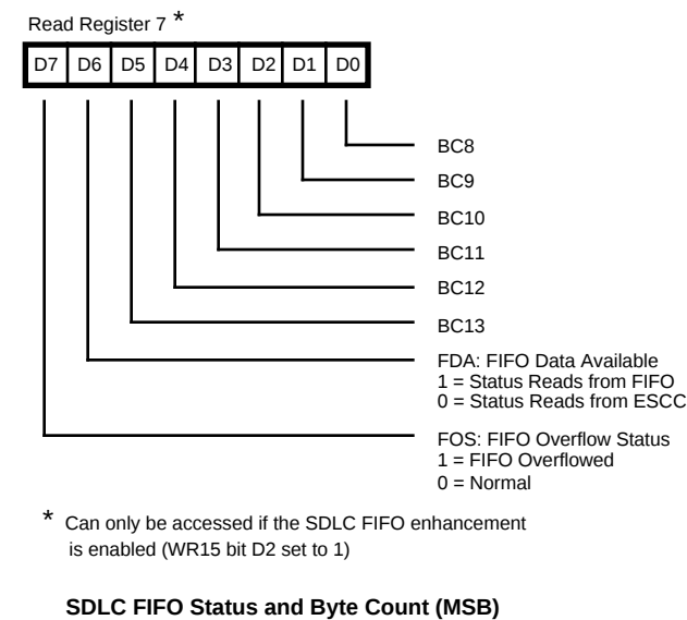
Figure 5-24. Read Register 7 (Not on NMOS)
