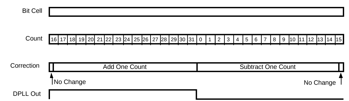
Figure 3-6. DPLL in NRZI Mode
