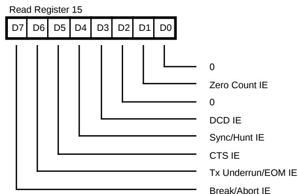
Figure 5-28. Read Register 15
