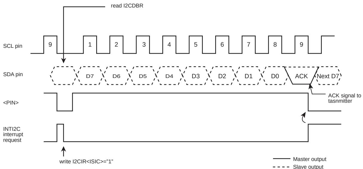
Figure 20-12 &lt;BC[2:0]&gt;= "000", &lt;ACK&gt;= "1" (Receiver Mode)
