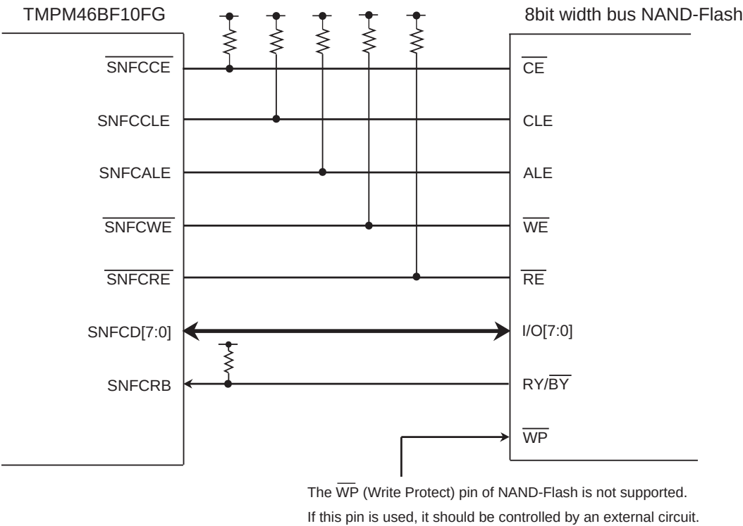
Figure 11-5 Connection Example
