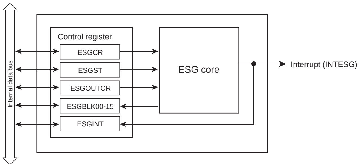
Figure 14-1 Block diagram of the ESG
