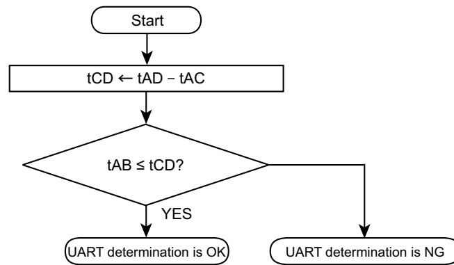
Figure 26-7 Serial operation mode determination flow chart
