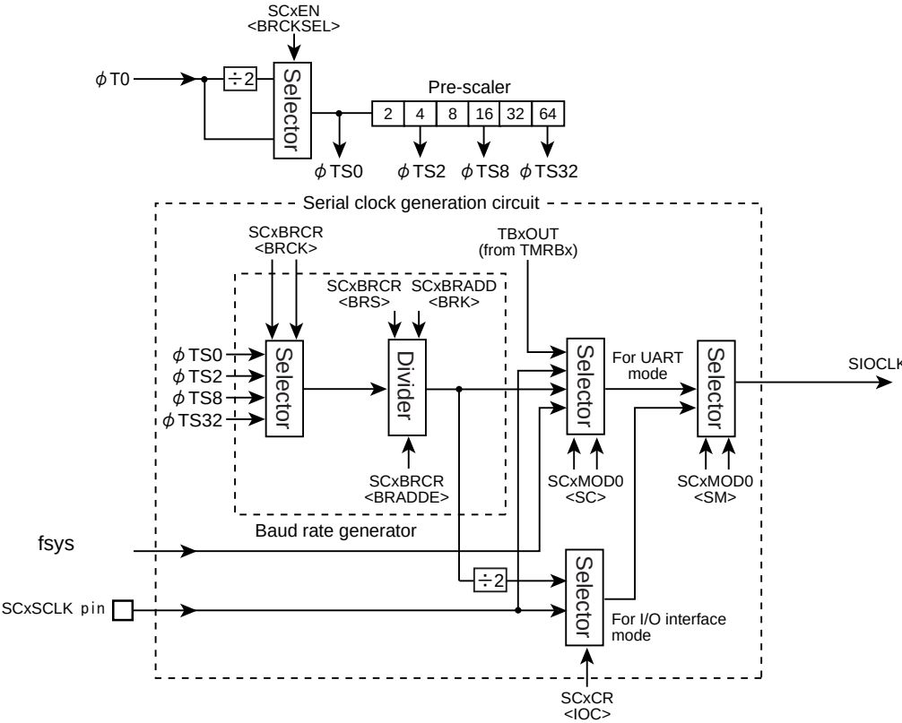
Figure 18-2 Serial clock generation circuit block diagram
