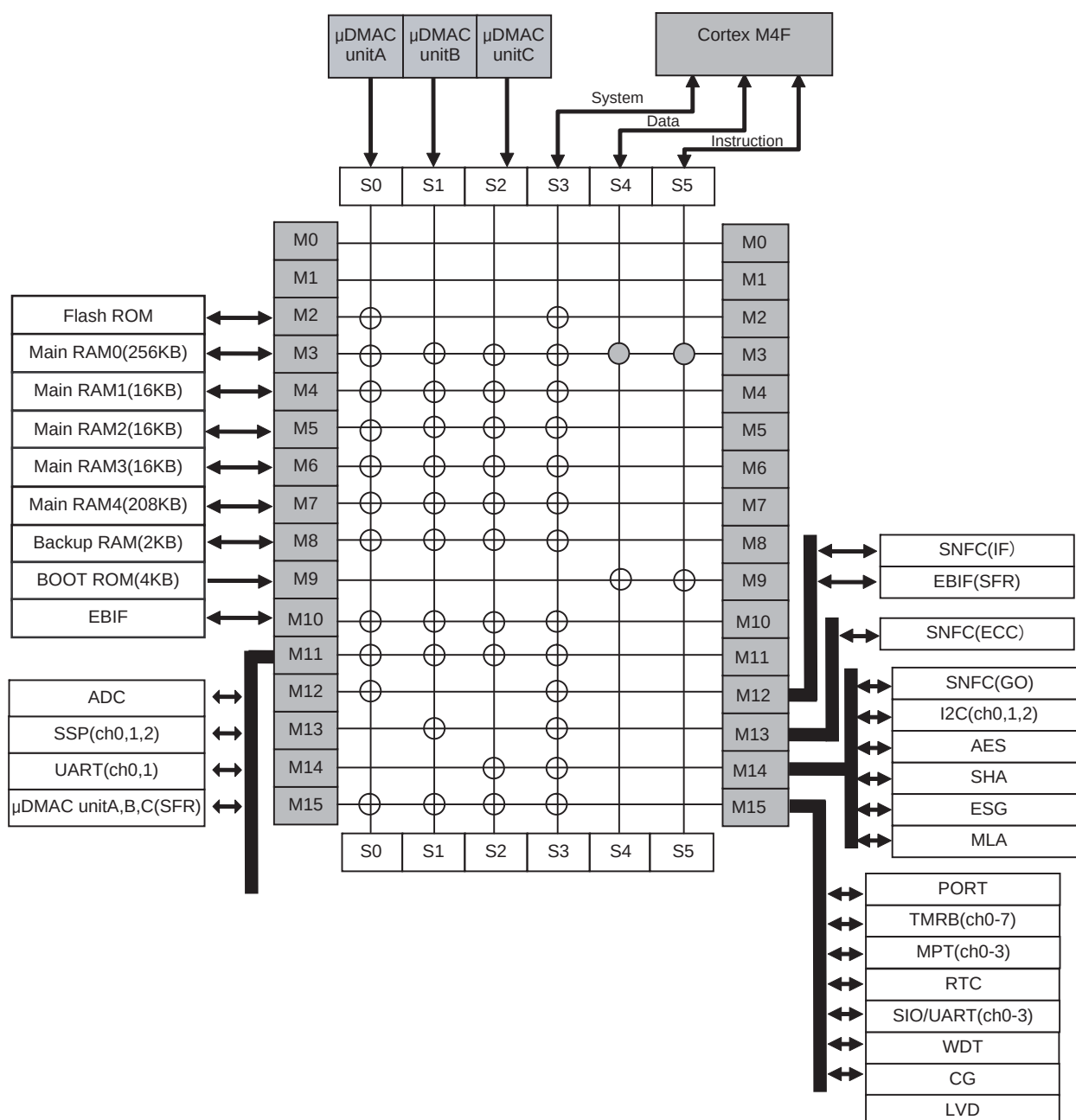
Figure 4-3 Bus Matrix of TPM46BF10FG
