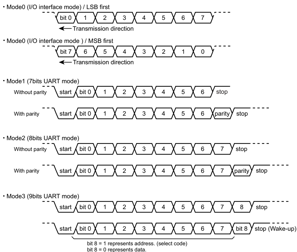
Figure 18-3 Data Format
