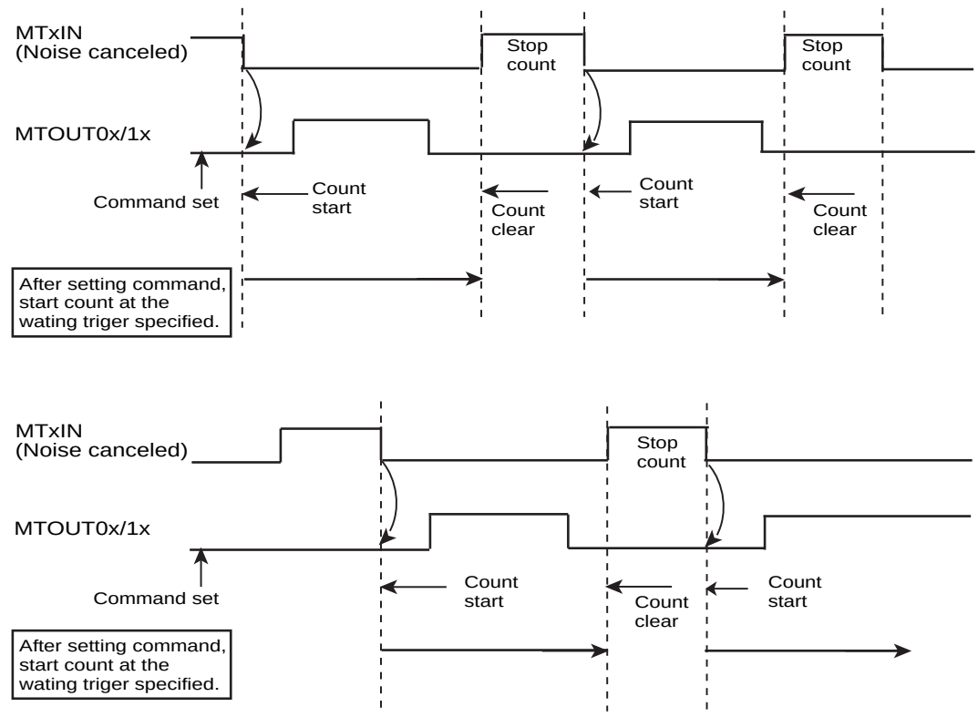
Figure 17-12 Trigger Start
