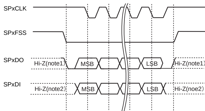
Figure 21-7 SPI frame format (single transfer, <SPO>="1" & <SPH>="0")
