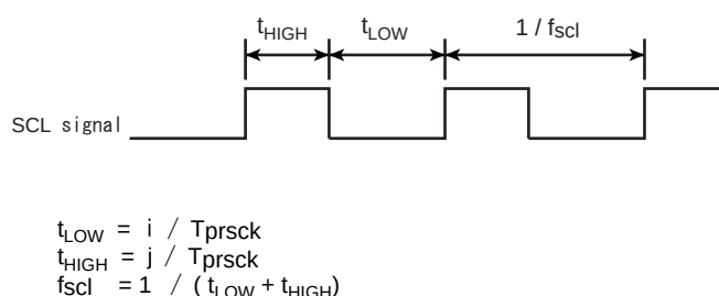
Figure 20-4 Clock source
