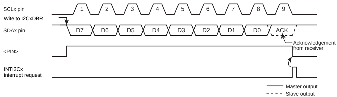
Figure 20-11 &lt;BC[2:0]&gt;= "000", &lt;ACK&gt;= "1" (Transmitter Mode)
