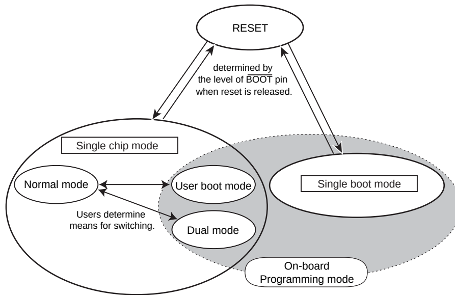
Figure 26-1 Mode transition
