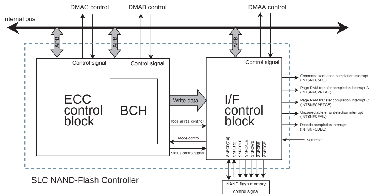
Figure 11-1 Block diagram
