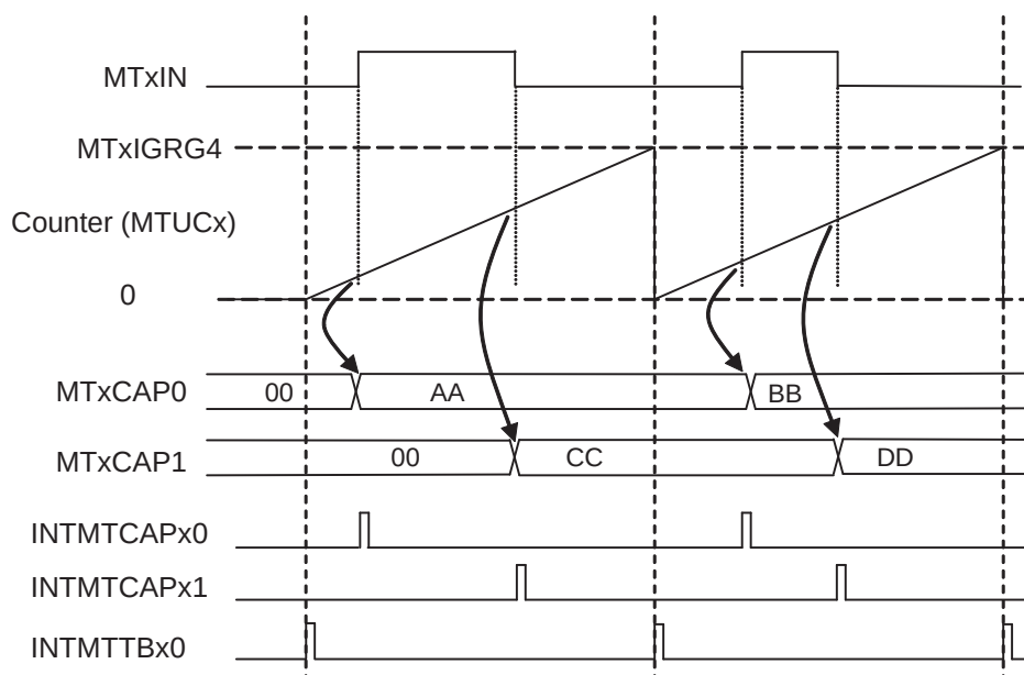
Figure 17-10 Capture operation
