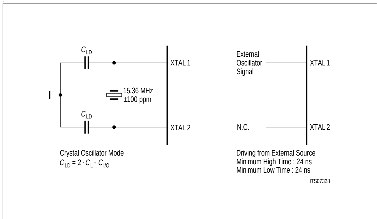
Figure 5-3 Recommended Oscillator Circuits
