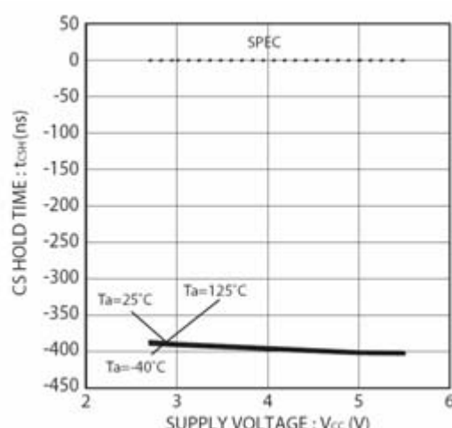
Figure 20. CS hold time t_{CSH}
