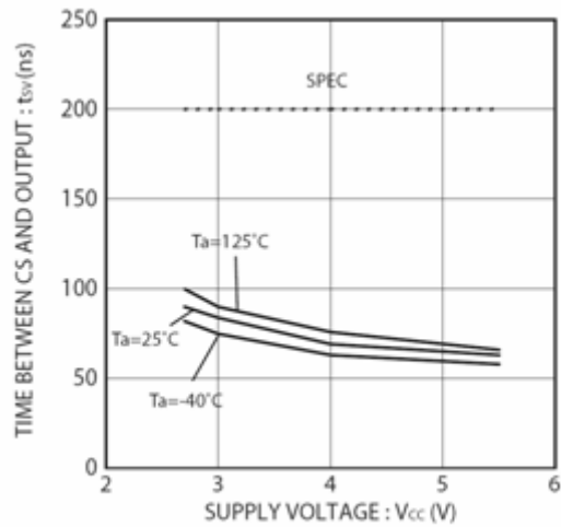
Figure 23. Time from CS to output establishment t_{SV}
