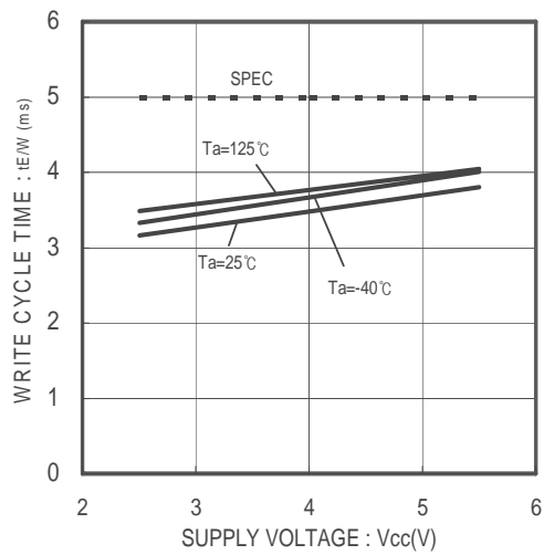
Figure 26. Write cycle time t_{E/W} (BR93H66RFVM-WC)
