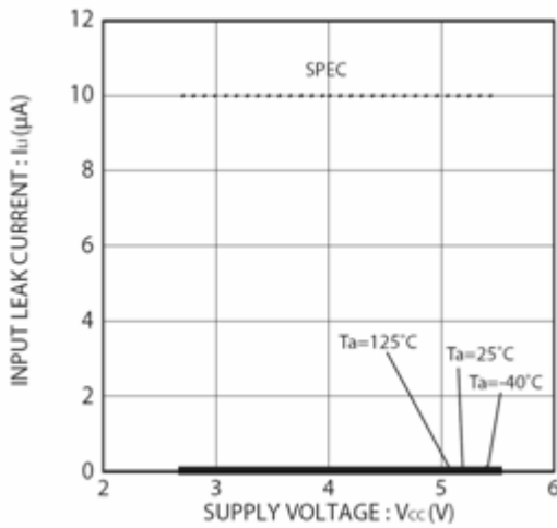
Figure 7. Input leak current I_{LI} (CS, SK, DI)
