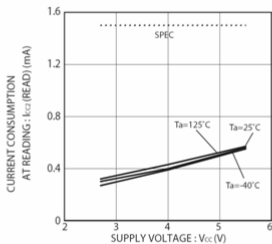
Figure 10. Consumption current at READ Operation ICC2 (READ, fSK=1.25MHz)
