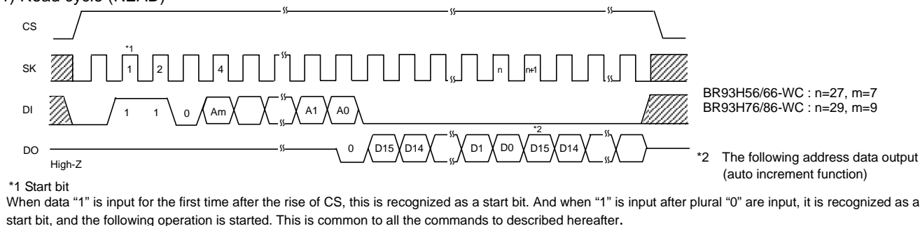
Figure 28. Read cycle
