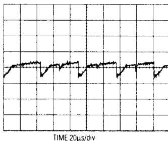
REGULATOR 6 OUTPUT RIPPLE UNFILTERED
