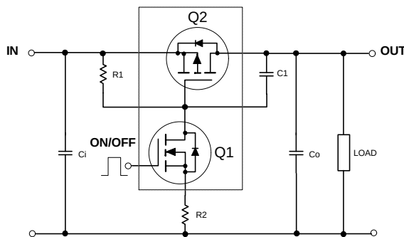
APPLICATION CIRCUIT
