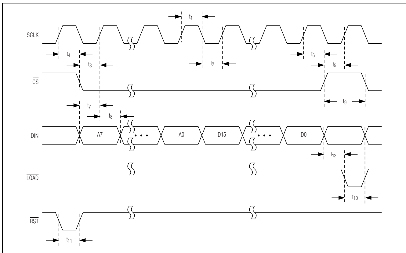
Figure 5. Serial-Interface Timing
