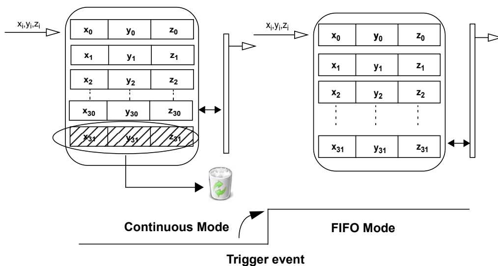
Figure 8. Continuous-to-FIFO mode
