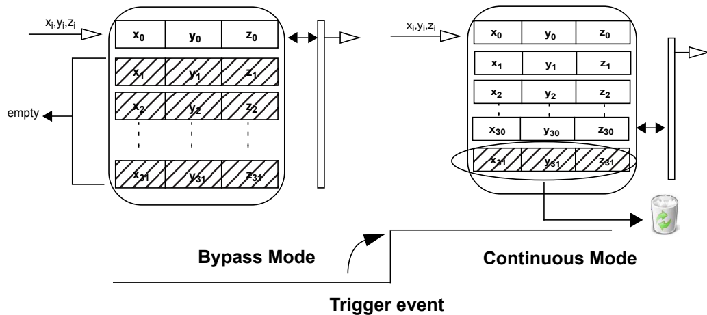
Figure 10. Bypass-to-continuous mode
