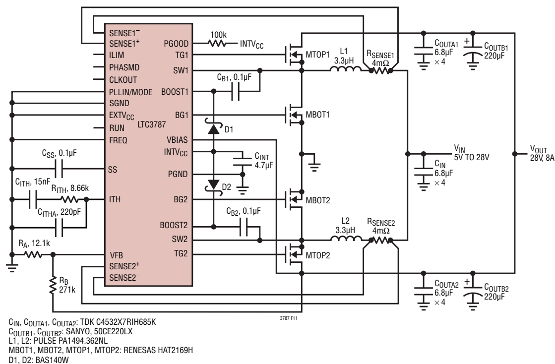
Figure 11. High Efficiency 2-Phase 28V Boost Converter
