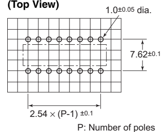
PCB Dimensions (Top View)
