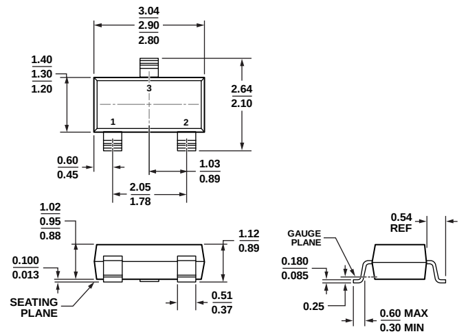
Figure 10. 3-Lead Small Outline Transistor Package [SOT-23] (RT-3)
