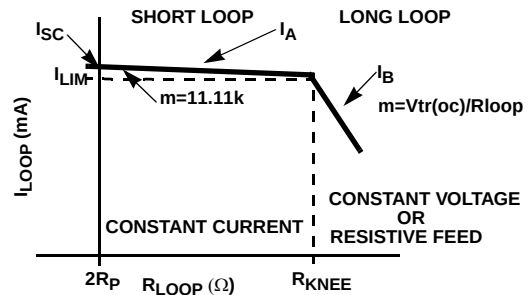
FIGURE 3. I_{\text{LOOP}} vs. R_{\text{LOOP}} LOAD CHARACTERISTIC
