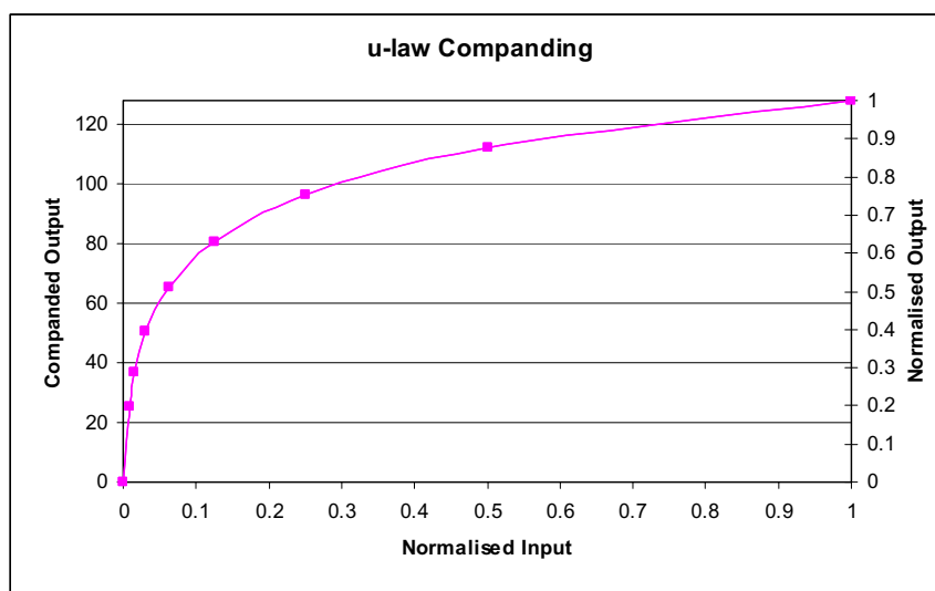
Figure 28 u-Law Companding
