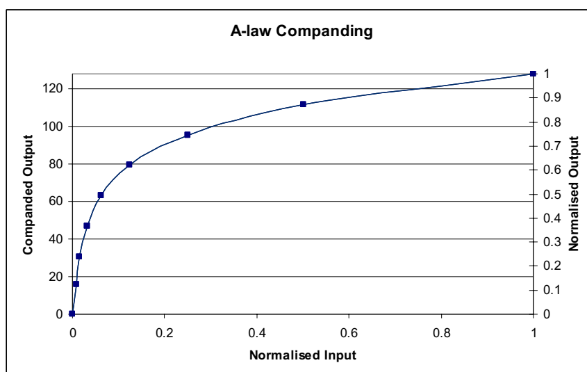
Figure 29 A-Law Companding
