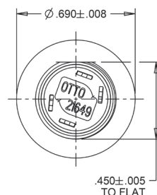
Threaded Case Terminal Detail
