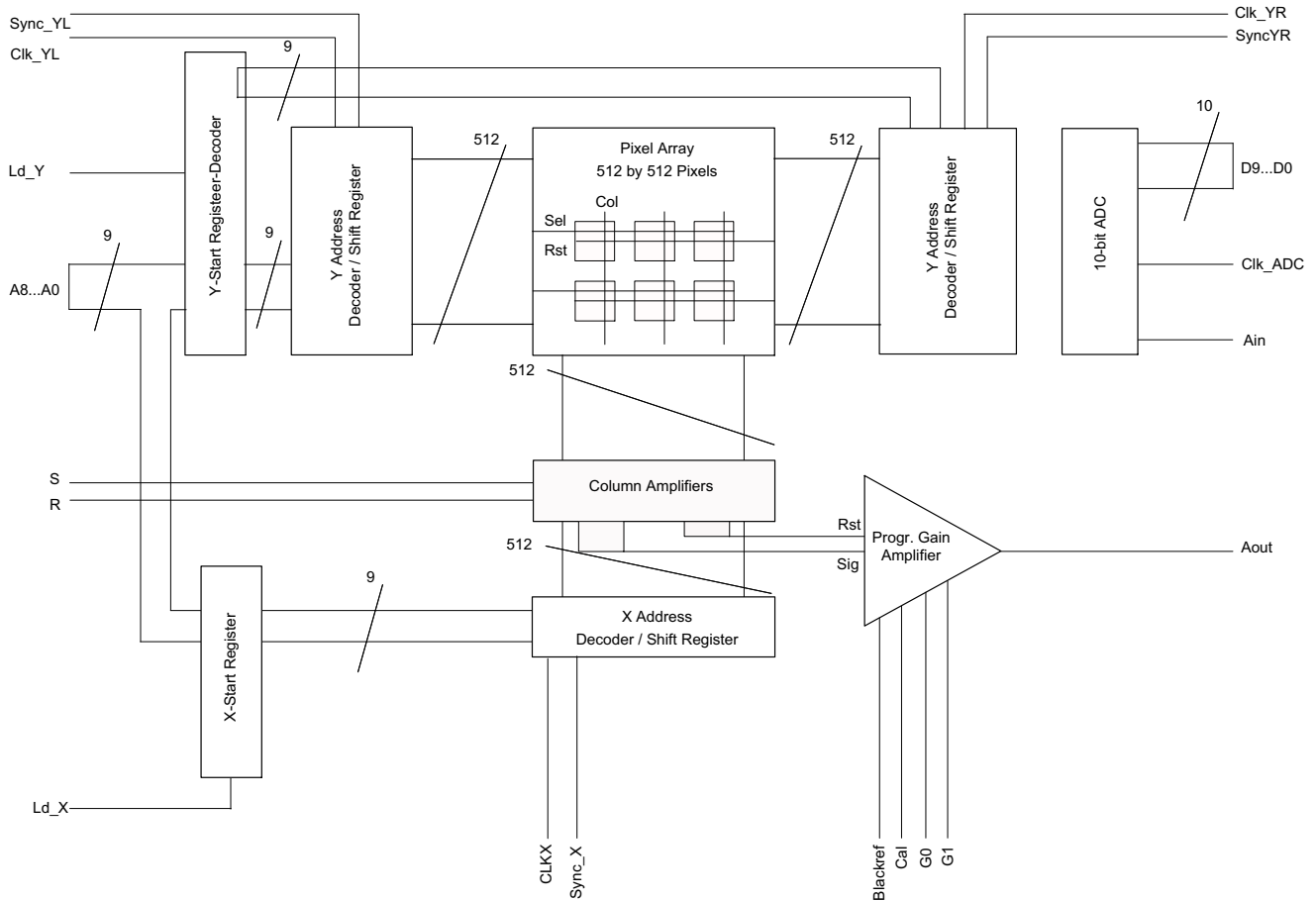
Figure 7. STAR250 Schematic
