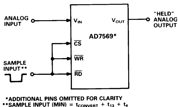
Figure 29. Infinite Sample-and-Hold
