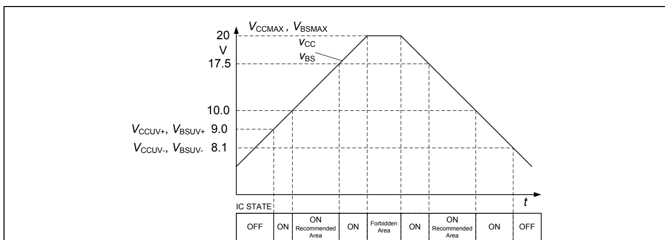
Figure 12 Operating areas (MOSFET UVLO levels)
