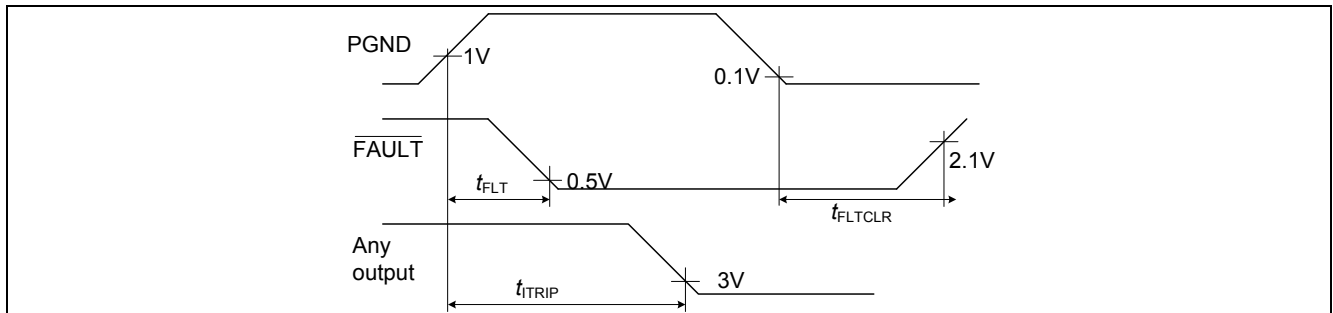
Figure 13 ITRIP-Timing
