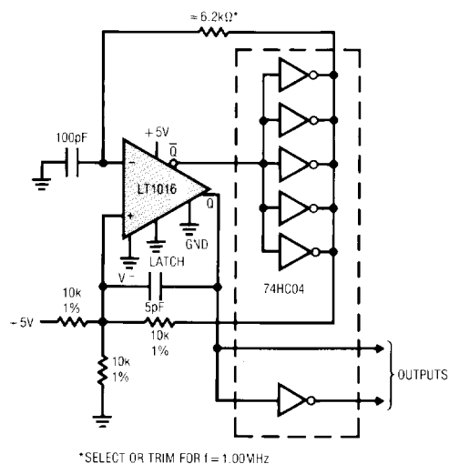
Single Supply Precision RC 1MHz Oscillator
