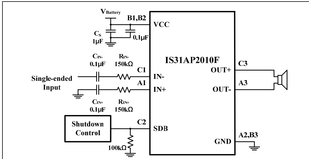
Figure 2 Typical Application Circuit (Single-ended Input)
