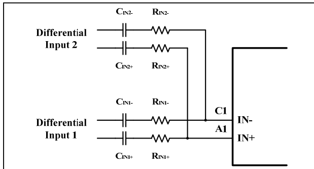
Figure 9 Summing Two Differential Inputs
