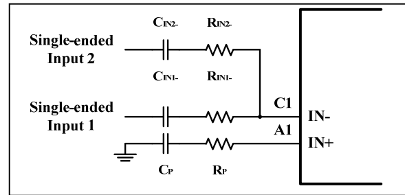
Figure 11 Summing Two Single-Ended Inputs
