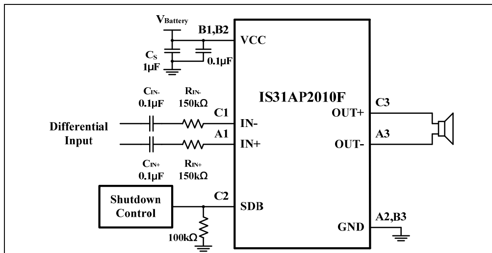
Figure 1 Typical Application Circuit (Differential Input)
