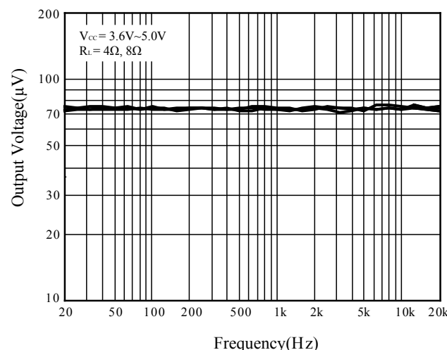
Figure 8 Noise
