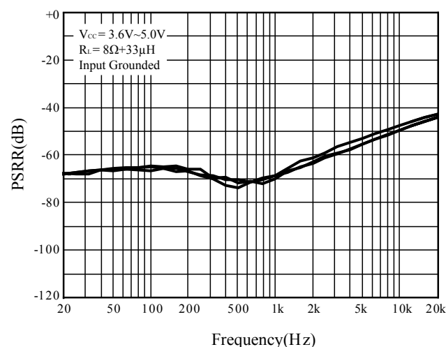
Figure 7 PSRR
