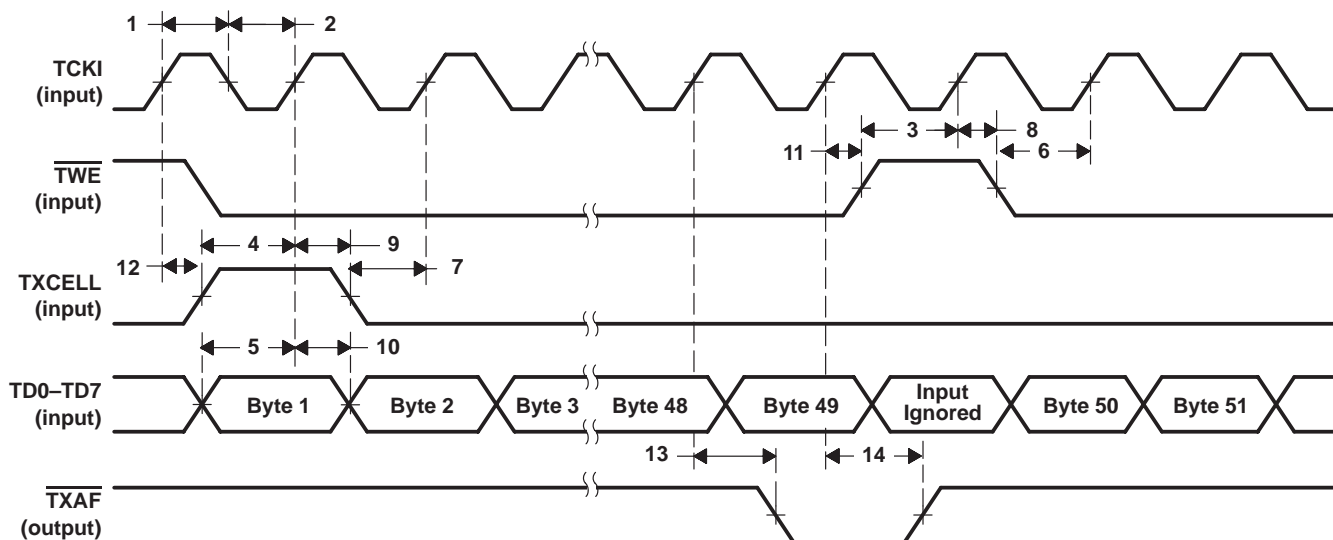
Figure 4. Transmit-Cell Interface
