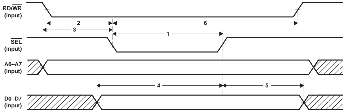
Figure 2. Controller-Interface Write Cycle
