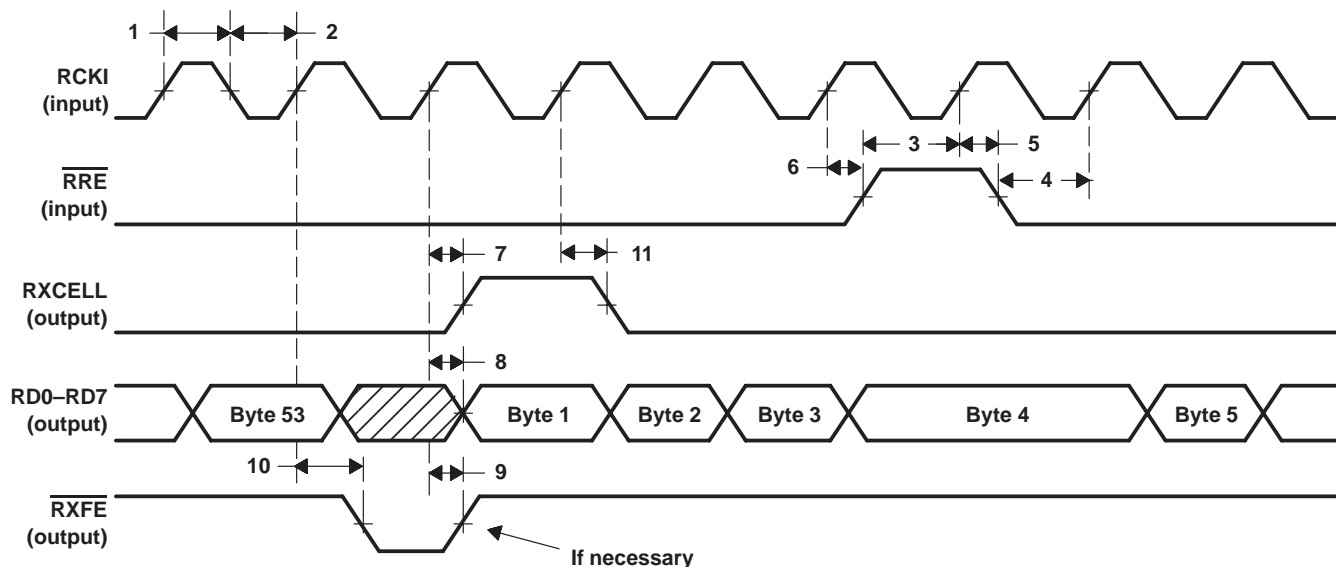
Figure 3. Receive-Cell Interface
