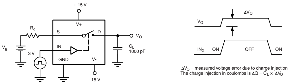
Figure 3. Charge Injection
