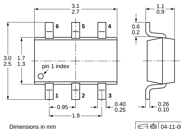
Fig 18. Package outline PIMD3 (SOT457/SC-74)
