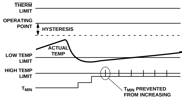
Figure 73. T_{MIN} Adjustments Limited by the High Temperature Limit
