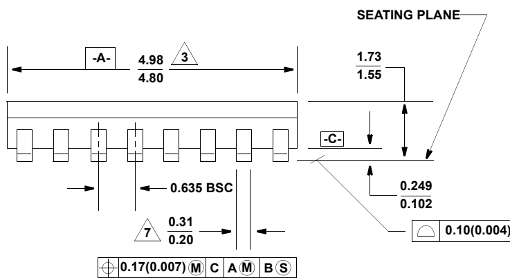
SIDE VIEW 1
