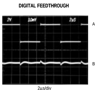
A: D0...D7 = 100kHz, 4Vp-p B: VOUT, 10mV/div LDAC = CS = HIGH
