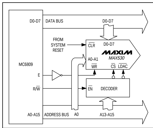
Figure 7. 8-Bit and 16-Bit \mu P Interface
