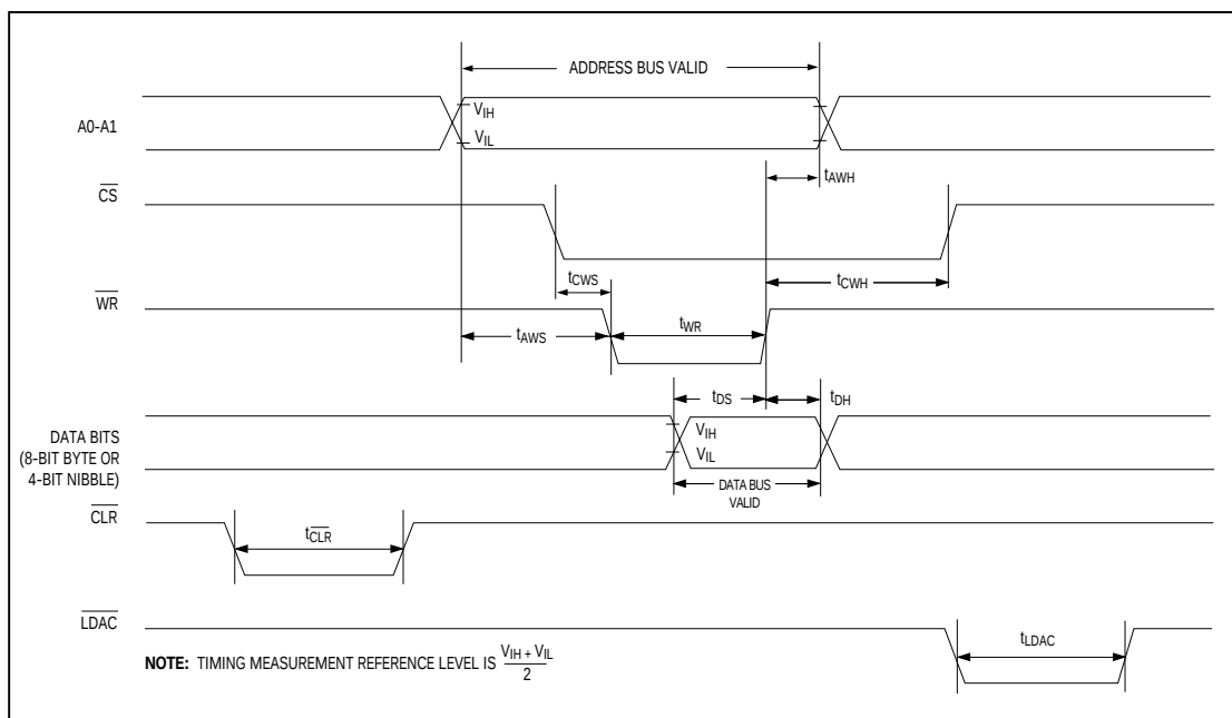
Figure 4. MAX530 Write-Cycle Timing Diagram
