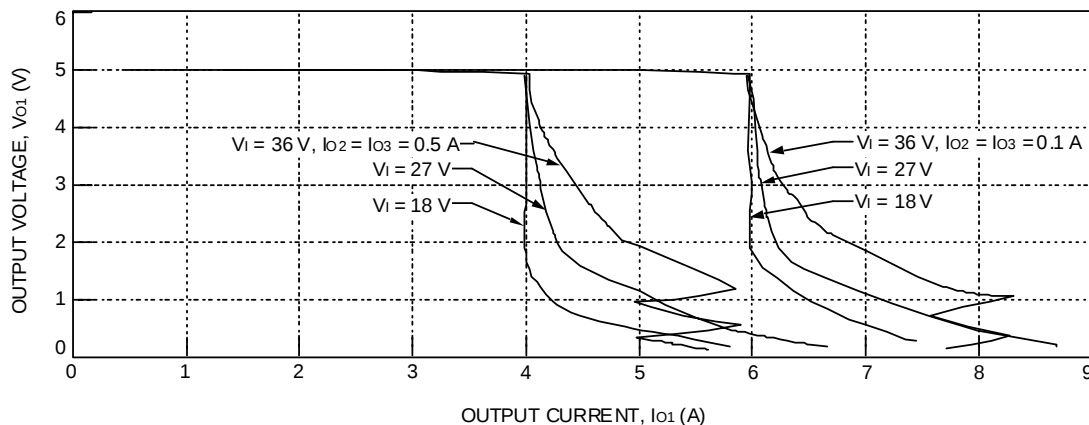
Figure 9. DC025ABK-M Typical 5 V Output Characteristics
