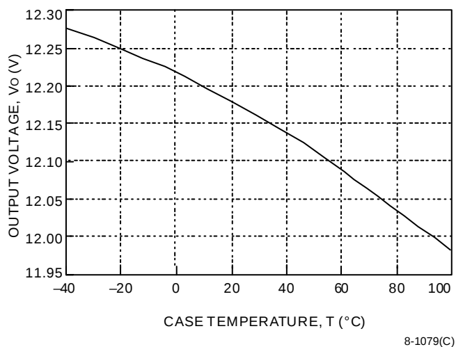
Figure 3. DC025 Triple Output-Series Typical Output Voltage Variation of 12 V Output Over Ambient Temperature Range
