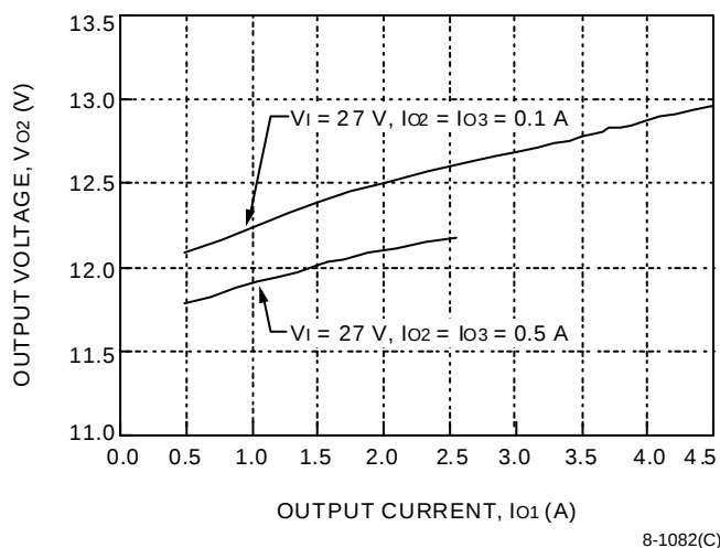
Figure 6. DC025ABK-M Typical Cross Regulation with Respect to I_{o1}
