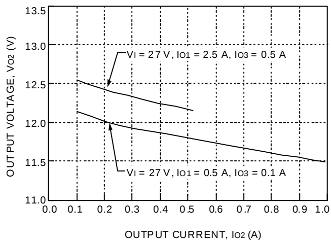
Figure 5. DC025ABK-M Typical Load Regulation
