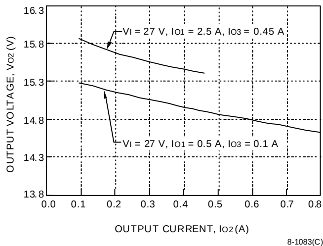
Figure 7. DC025ACL-M Typical Load Regulation
