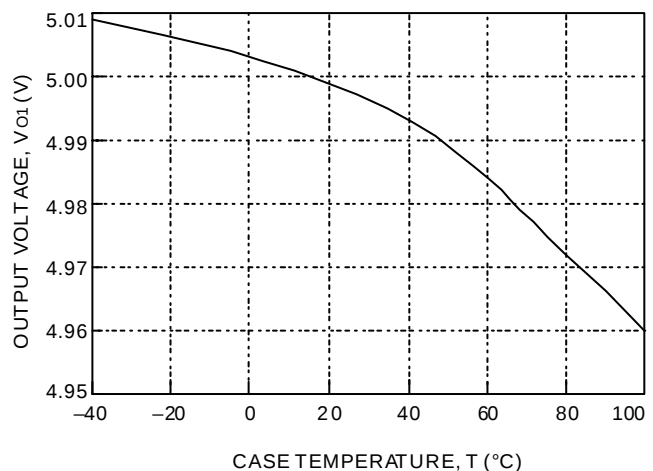
Figure 2. DC025 Triple Output-Series Typical Output Voltage Variation of 5 V Output Over Ambient Temperature Range
