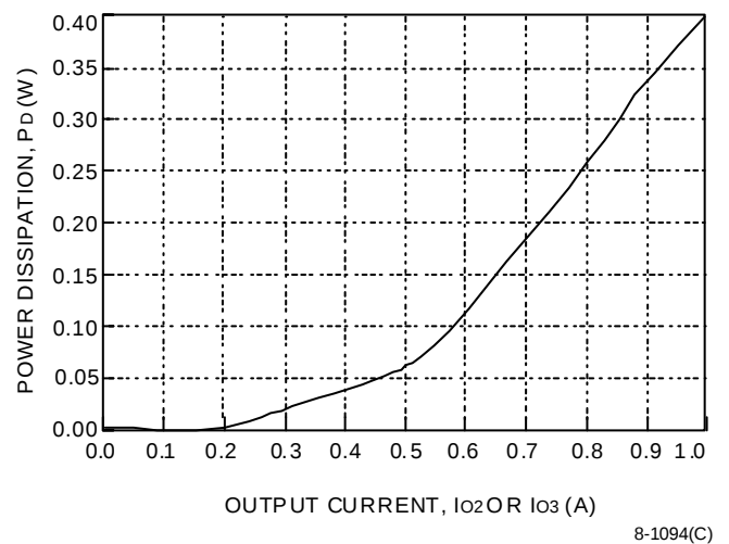
Figure 26. DC025ABK-M, Losses Associated with \pm 12 V Output, P_{s2}/P_{s3}
