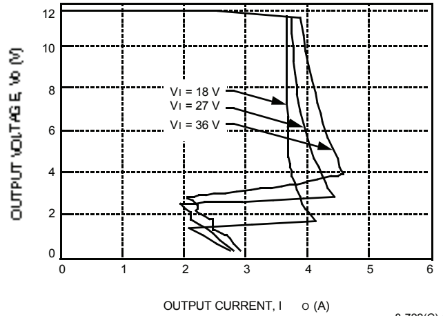
Figure 3. CC030B Typical Output Characteristics
