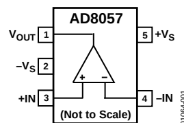
Figure 1. RT-5 (SOT-23)
