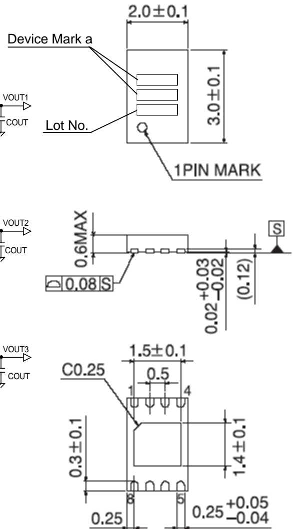
Fig.2 Package Dimensions (unit:mm)
