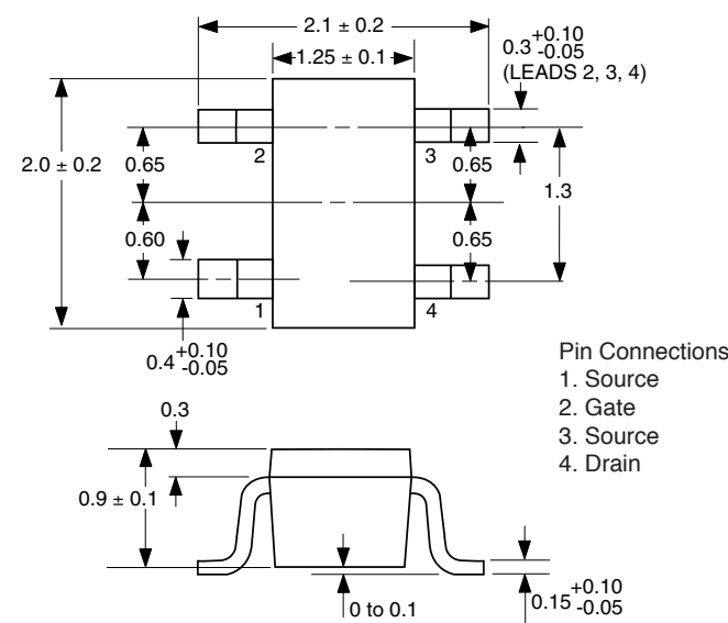
PACKAGE OUTLINE 18
