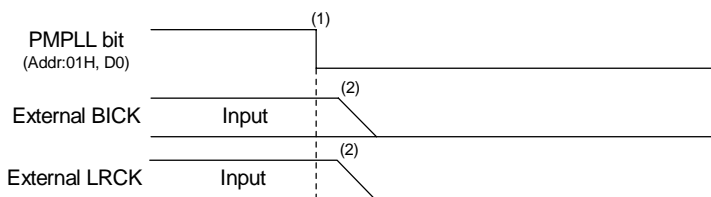
Figure 85. Clock Stopping Sequence (2)
