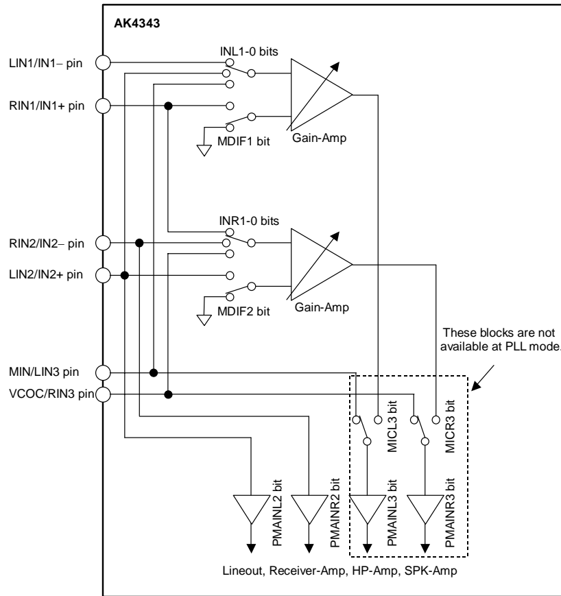
Figure 31. Input Selector
