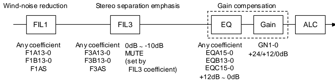
Figure 32. Digital EQ/HPF/LPF
