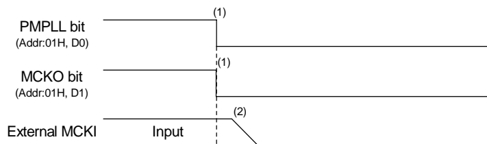
Figure 86. Clock Stopping Sequence (3)
