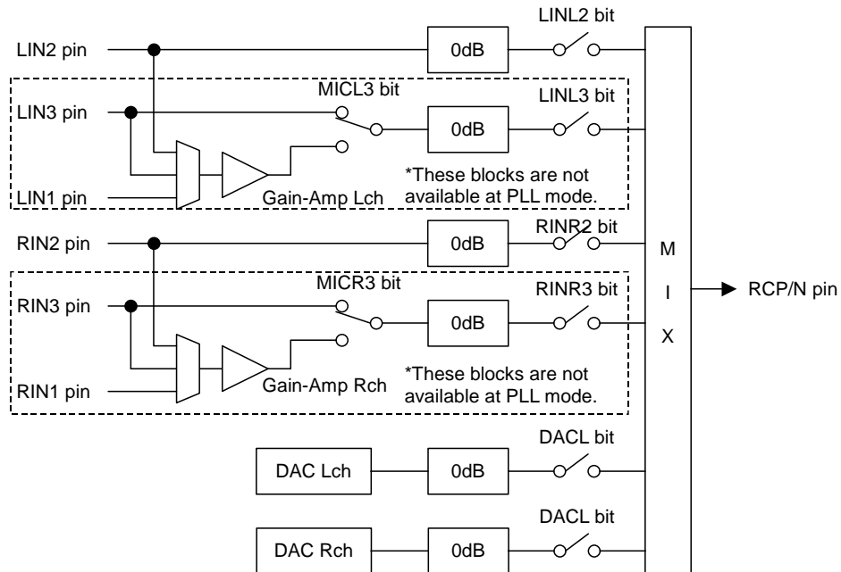
Figure 51. Receiver Mixing Circuit (AIN3 bit = "1", LOVL bit = "0")
