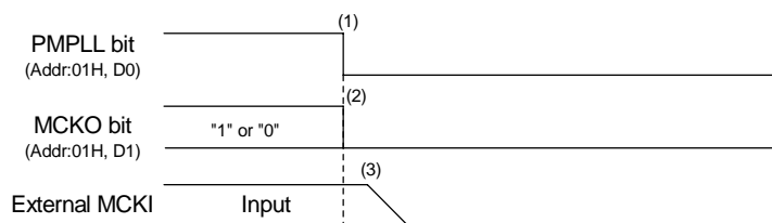
Figure 84. Clock Stopping Sequence (1)
