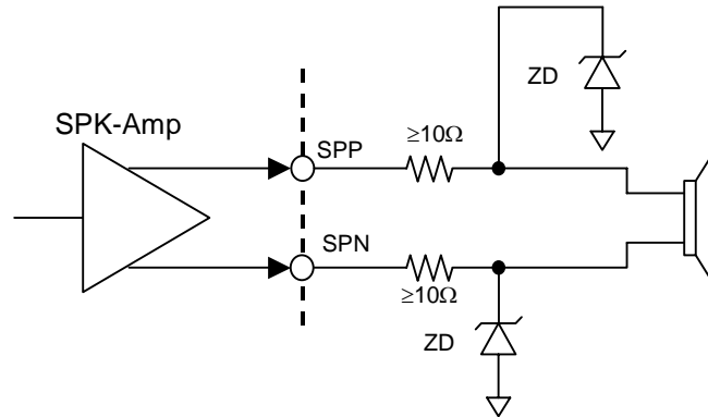
Figure 58. Speaker Output Circuit (Load Capacitance &gt; 30pF)
