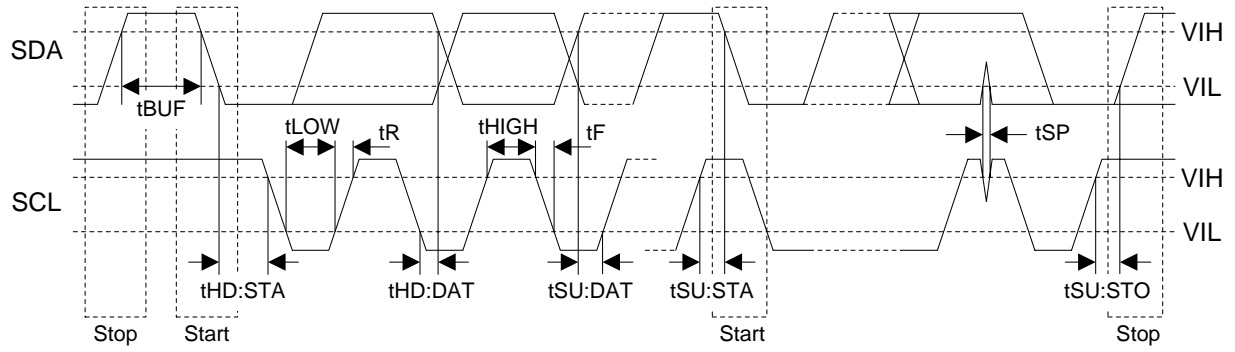
Figure 16. I²C Bus Mode Timing
