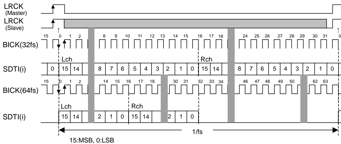
Figure 25. Mode 0 Timing (BCKP = "1", MSBS = "0")
