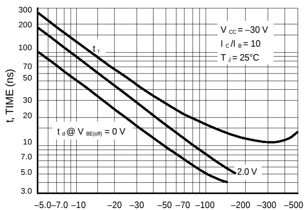
Figure 5. Turn-On Time
