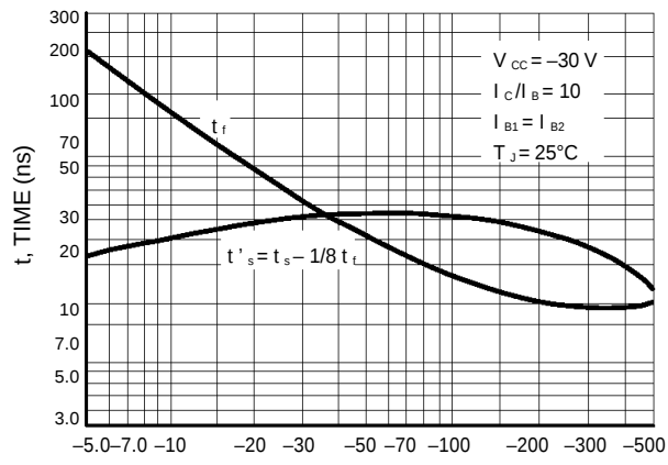
Figure 6. Turn-Off Time
