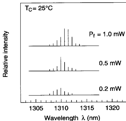
Lasing Wavelength (HL1321BF/DL/DM)
