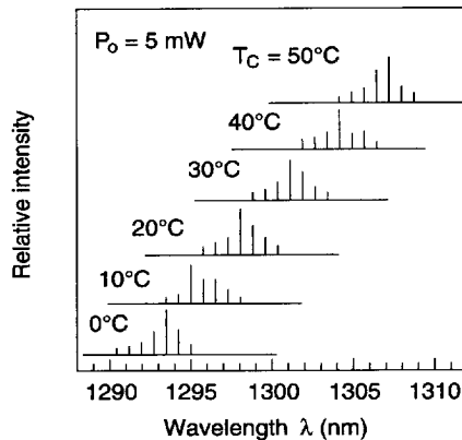
Lasing Wavelength Temperature Dependence (HL1321AC, HLP5400)
