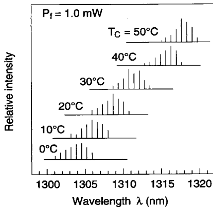
Lasing Wavelength Temperature Dependence (HL1321BF/DL/DM)
