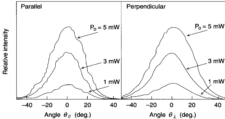
Far Field Pattern (HL1321AC, HLP5400)
