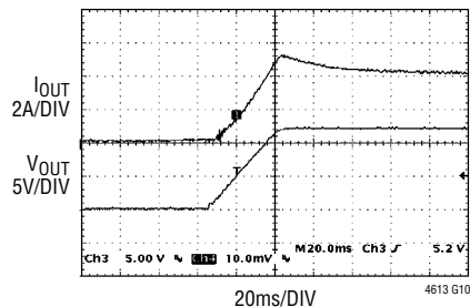
Start-Up with 24V_{IN} to 12V_{OUT} at I_{OUT} = 8A , T_A = -55^\circ C
