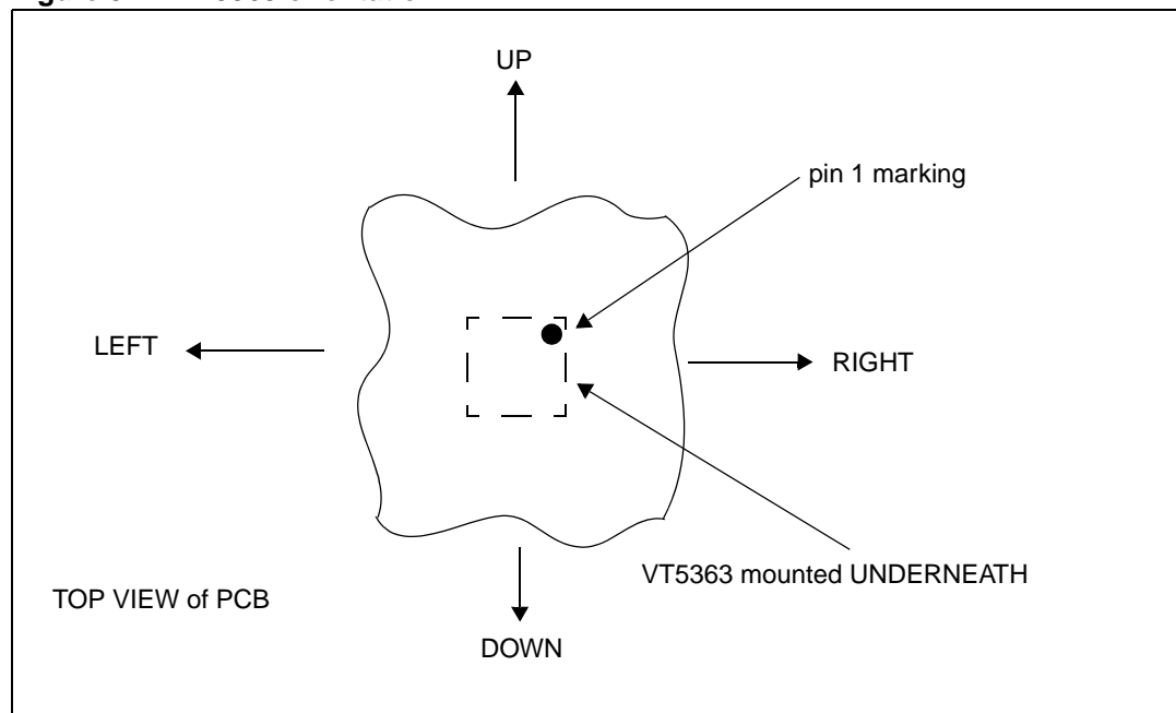
Figure 5. VT5363 orientation
