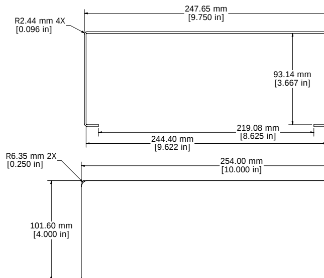
ASSEMBLY - SIDE VIEW (OPEN)
