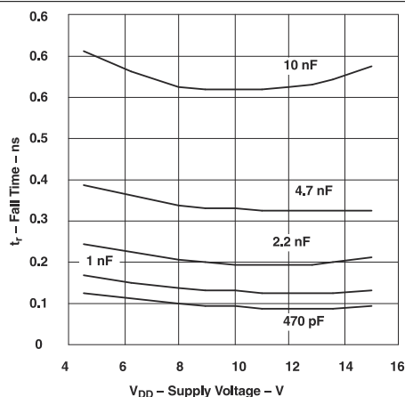
Figure 6-15. Fall Time vs Supply Voltage
