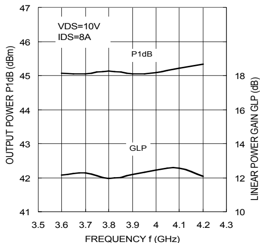
P1dB, GLP vs. f
