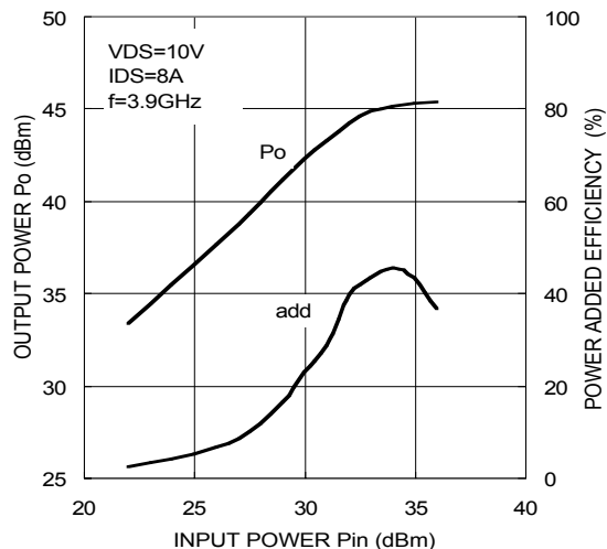
Po, P.A.E. vs. Pin
