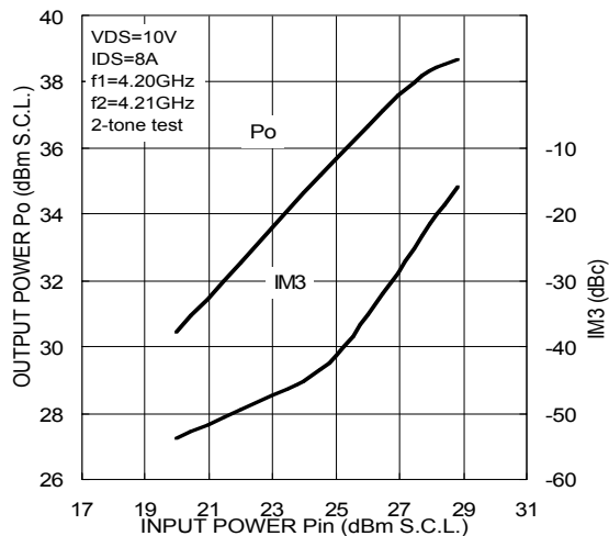
Po, IM3 vs. Pin
